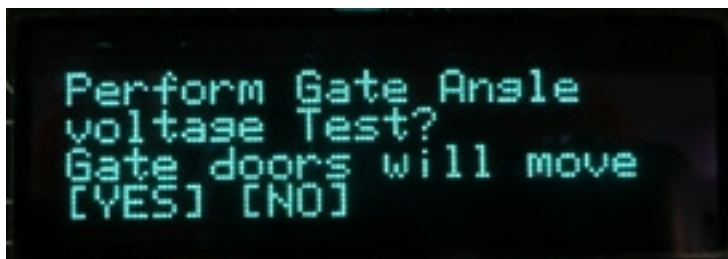
Figure 22 - Gate Angle voltage test menu
