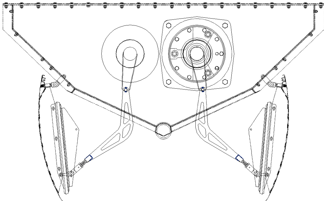
Figure 3 ~ Hopper gatebox and doors controlled by the actuator
